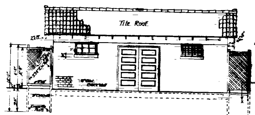
SIDE ELEVATION Scale 1/4\"/>
