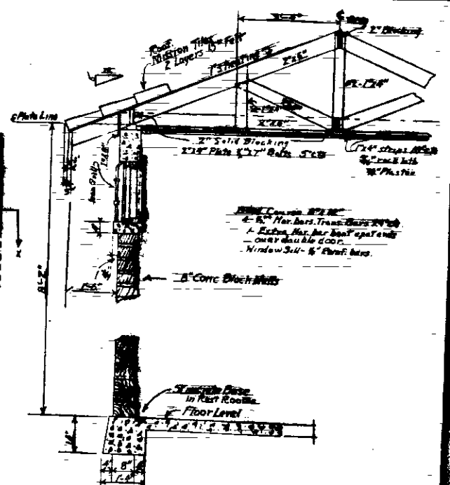
PART SECTION Scale 1/4\"/>
