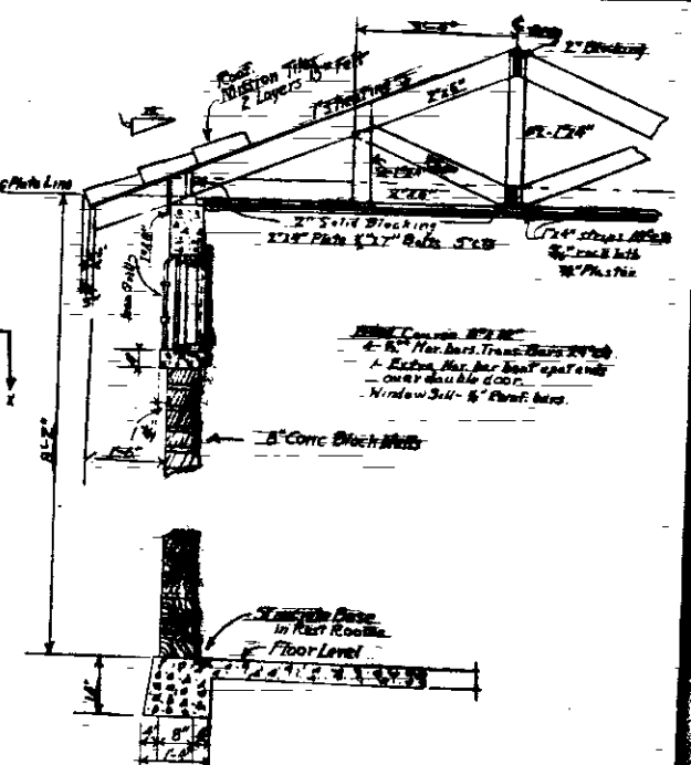
PART SECTION Scale 1/4\"/>
